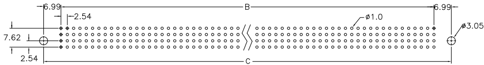
P.C. Board Layout
