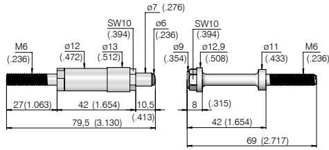
HSS-2513 (test probe) KT-2513 (contact terminal)
