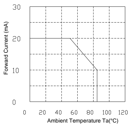
Derating
