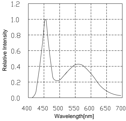
Spectral Distribution
