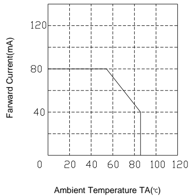
Derating
