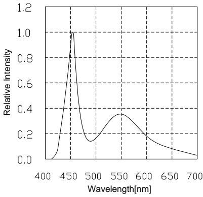
Spectral Distribution
