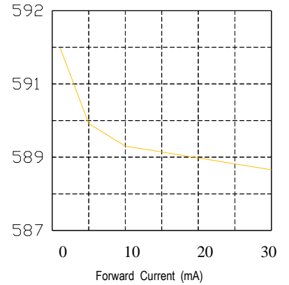
Forward Current vs. Dominant wavelength (Ta=25°C)
