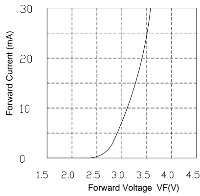
Forward Current vs. Forward Voltage (Ta=25° C)
