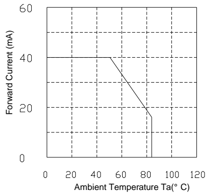
Derating
