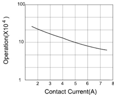
Life Curves
