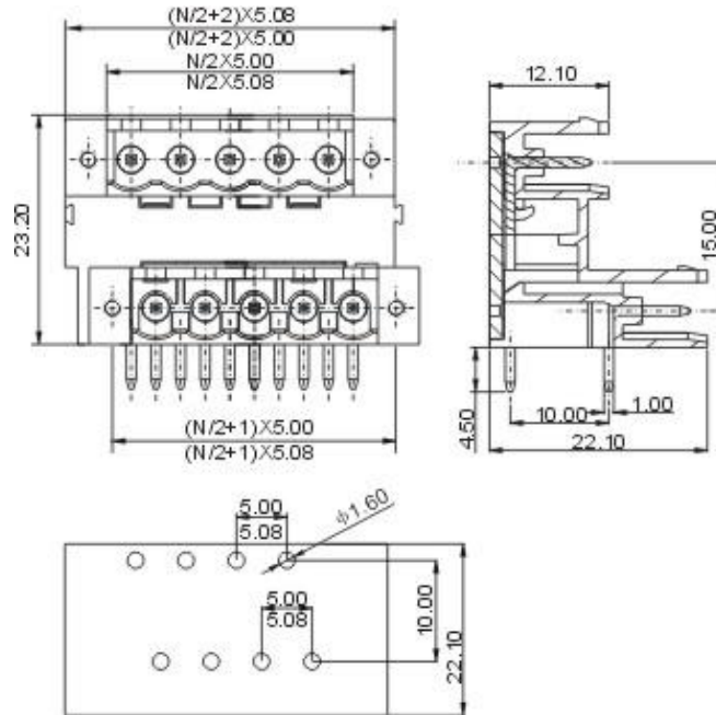
PCB LAYOUT
